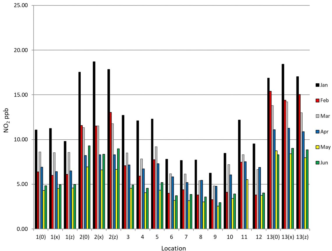
Figure 1: Passive NO 2 monitoring results, January to June
